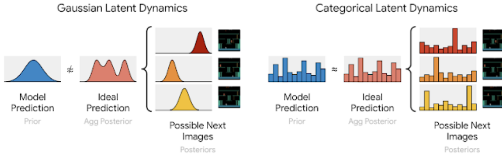
Figure 4: Image from official DreamerV2 blog, Gaussian and Categorical latent dynamics.
